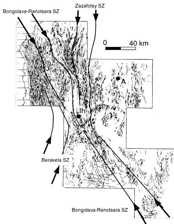
Fig. 6. Detailed foliation trajectories from Fig. 1 (sector 2, Ankaramena–Ihosi in text). Same legend as in Fig. 3. The heavy black lines define the limits of the Bongolava–Ranotsara SZ, Beraketa SZ, and Zazafotsy SZ. The density of brittle structures increases from north-east to south-east and disturb the interpretation of ductile structures.
